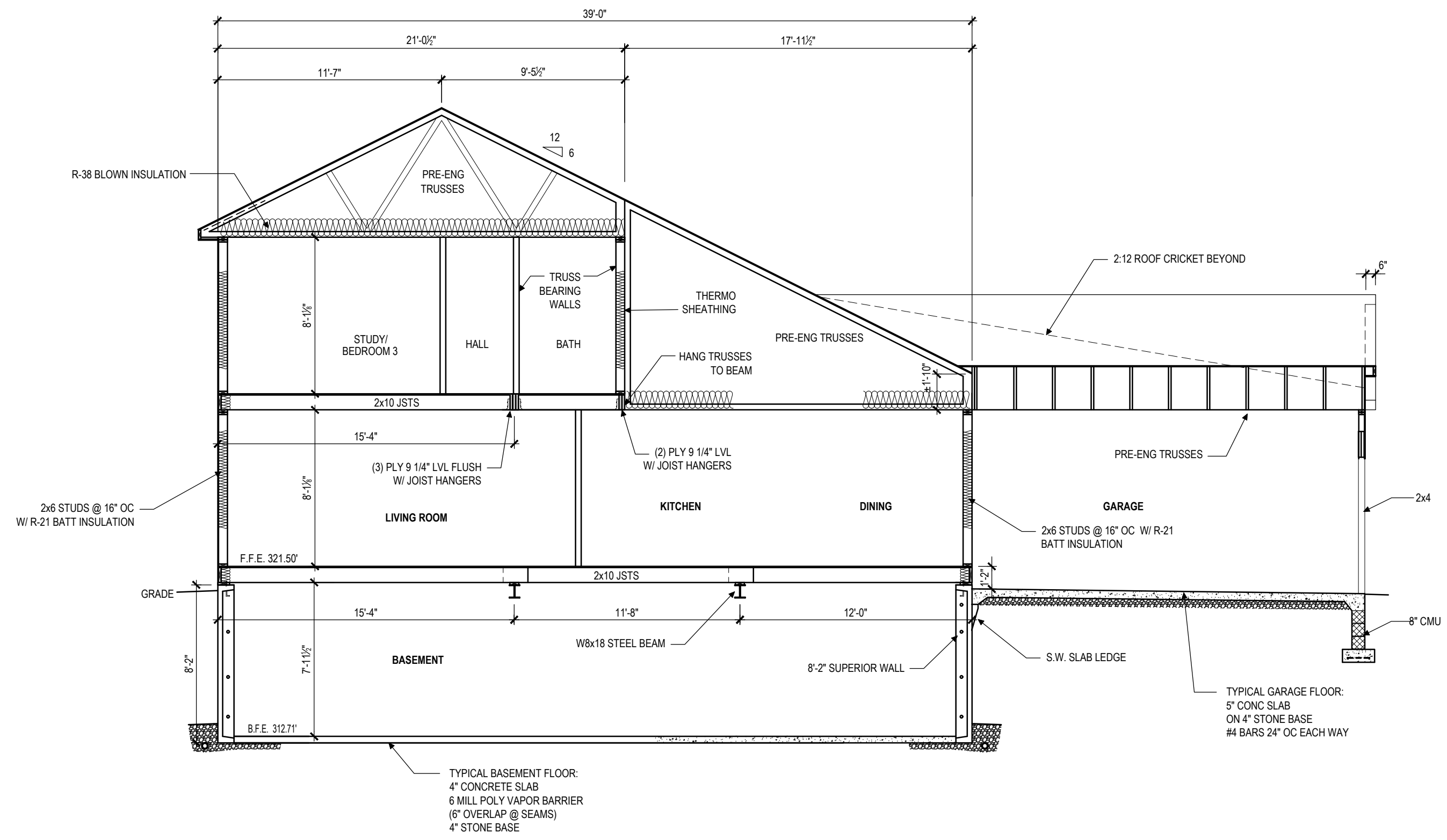
1 A305 OSPREY - SECTION 'A' SCALE: 3/16"=1'-0"
