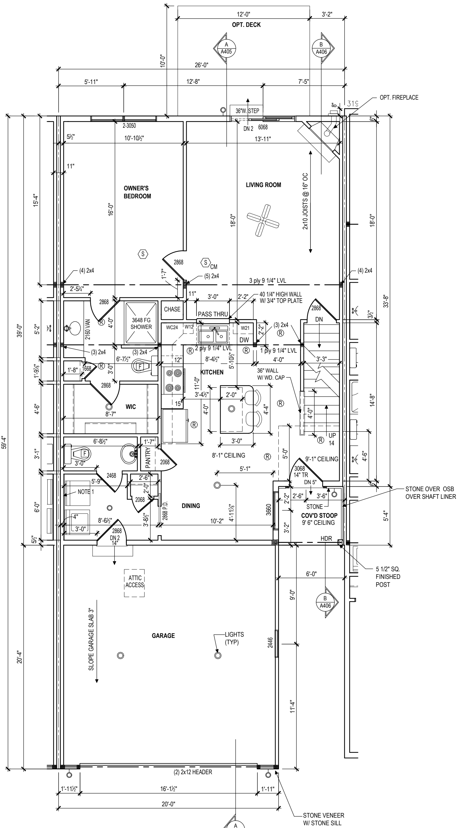
FIRST FLOOR PLAN 8'-1 1/8" WALL HEIGHT SCALE: 3/16"=1'-0"
