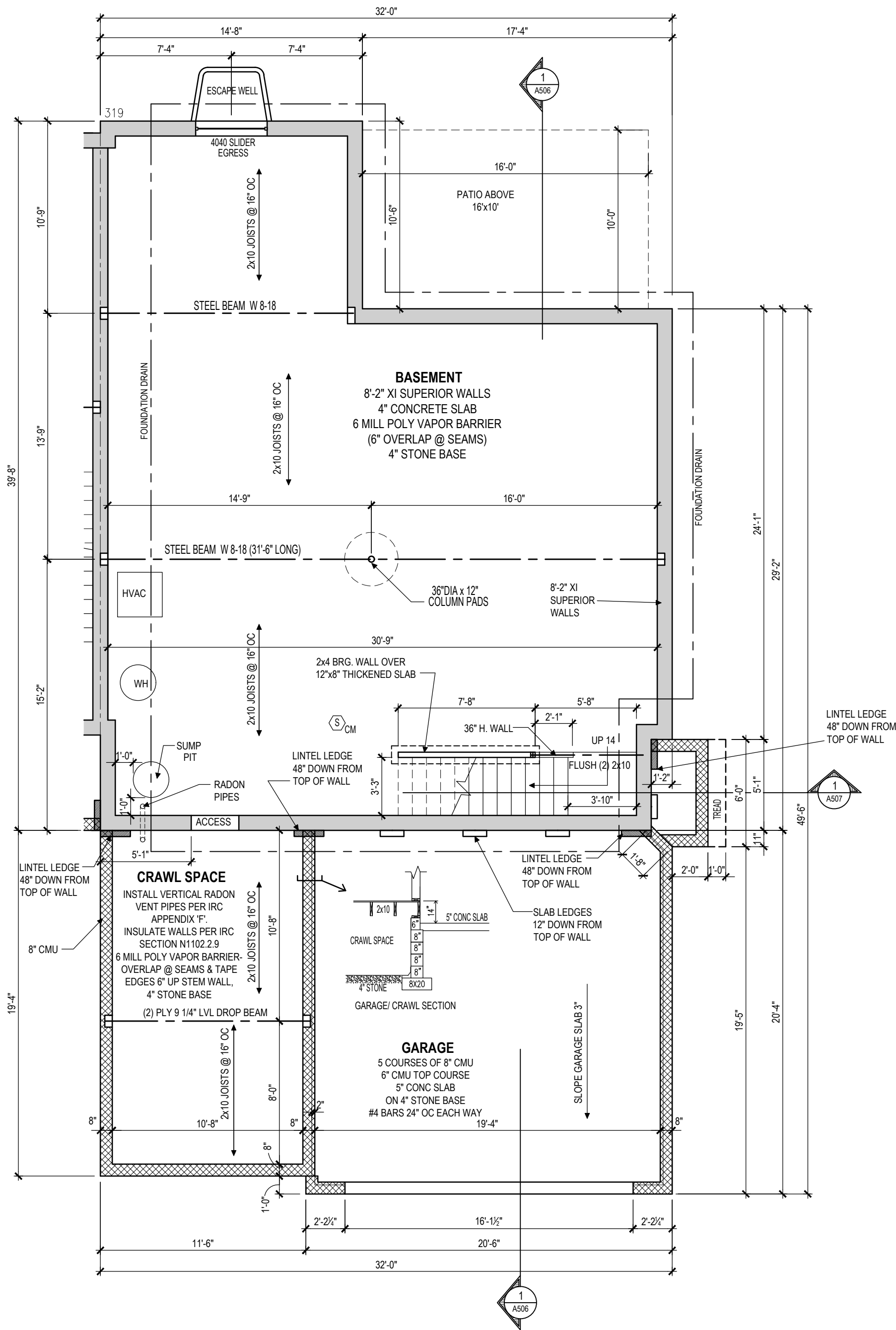
BASEMENT-FOUNDATION PLAN SCALE: 3/16"=1'-0"
