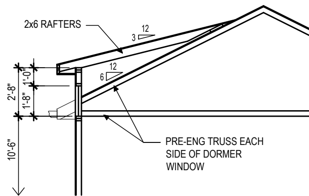
D A208 GARAGE DORMER SECTION SCALE: 3/16"=1'-0"
