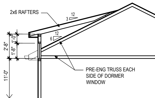
D A307 GARAGE DORMER SECTION SCALE: 3/16"=1'-0"
