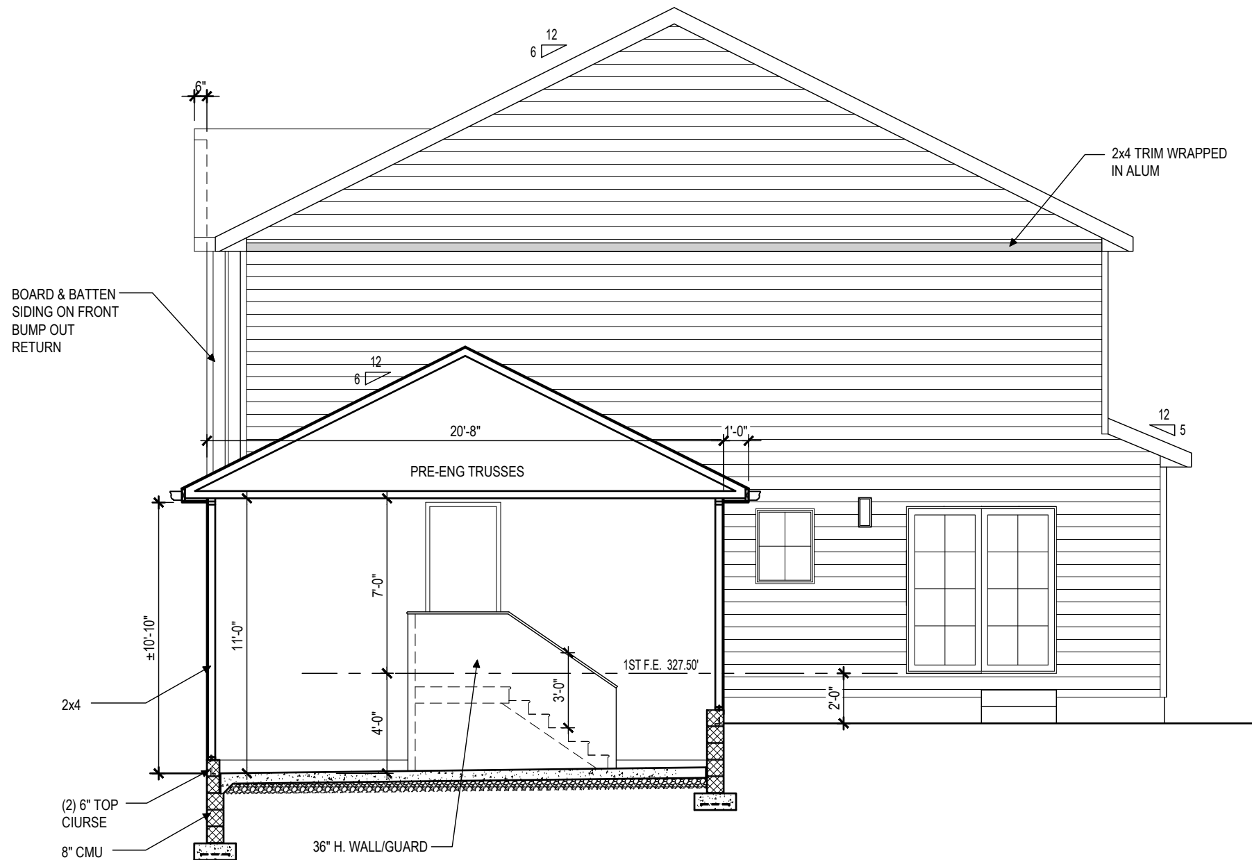
C A307 GARAGE SECTION / ELEVATION 'C' SCALE: 3/16"=1'-0"
