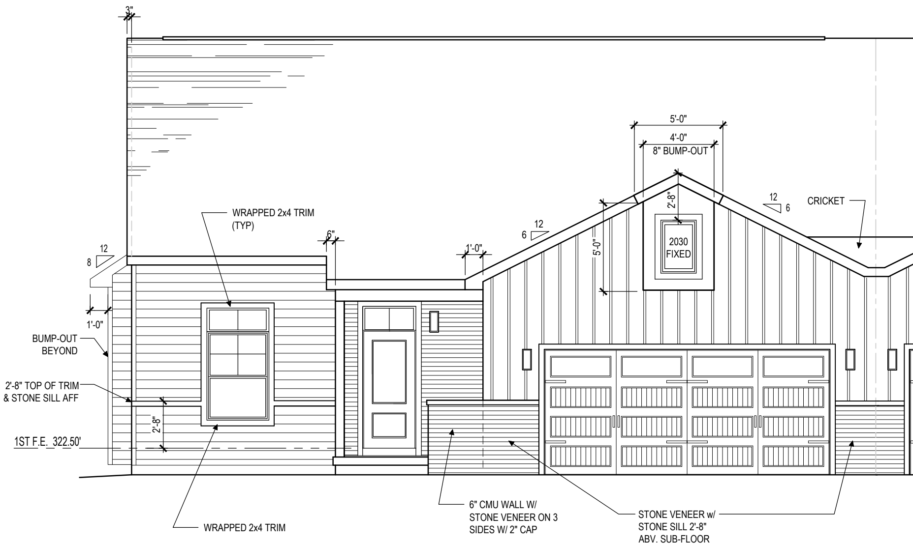
1 FRONT ELEVATION A203 SCALE: 3/16"=1'-0"
