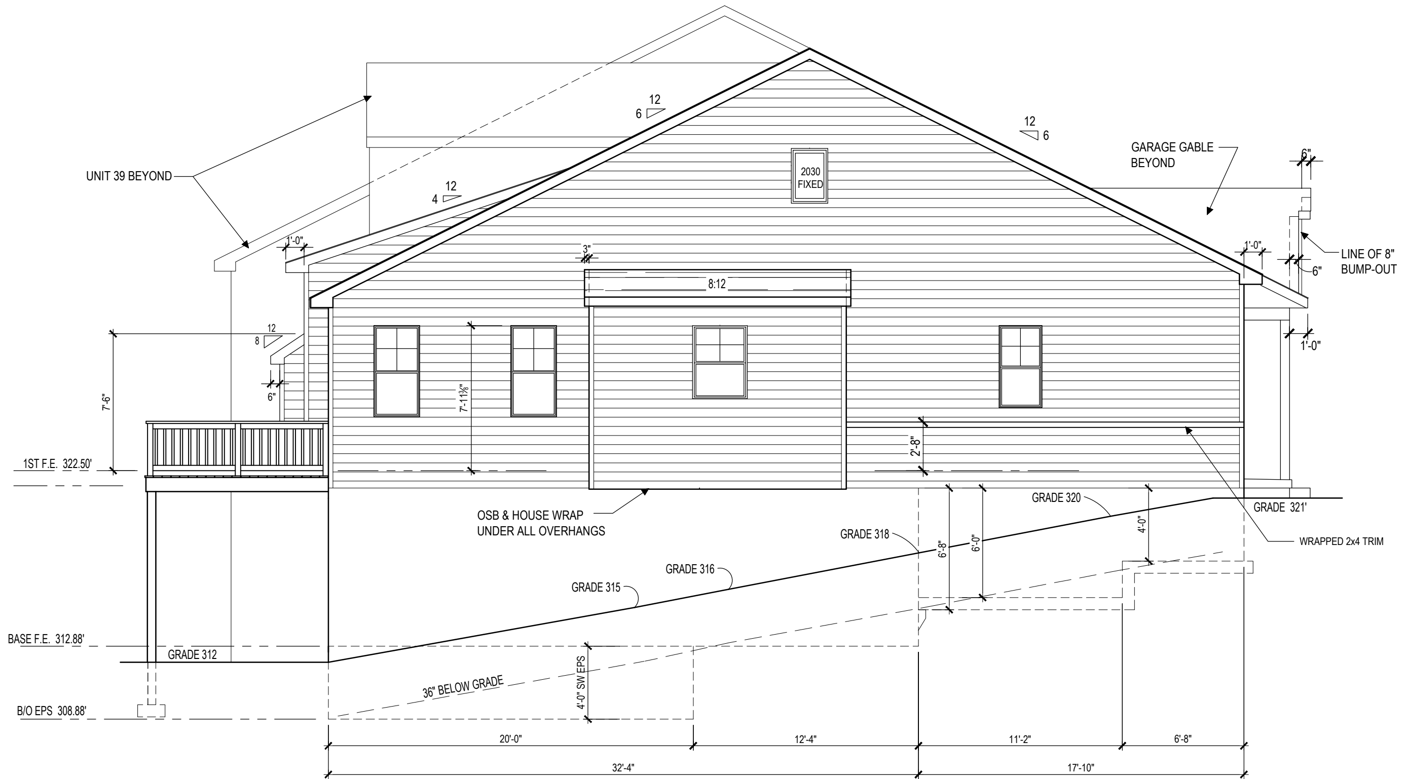
1 A204 SIDE ELEVATION SCALE: 3/16"=1'-0"
