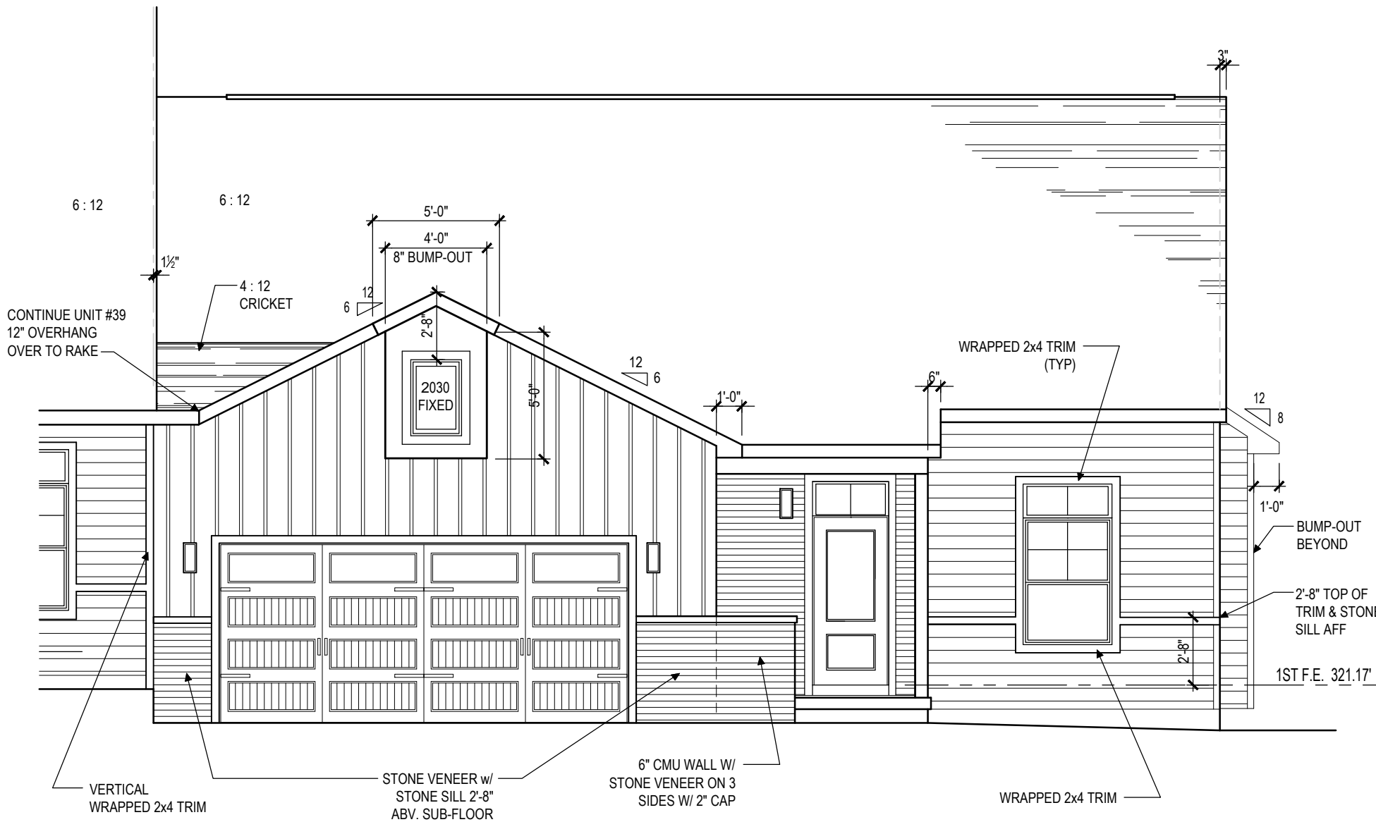
1 A403 FRONT ELEVATION SCALE: 3/16"=1'-0"
