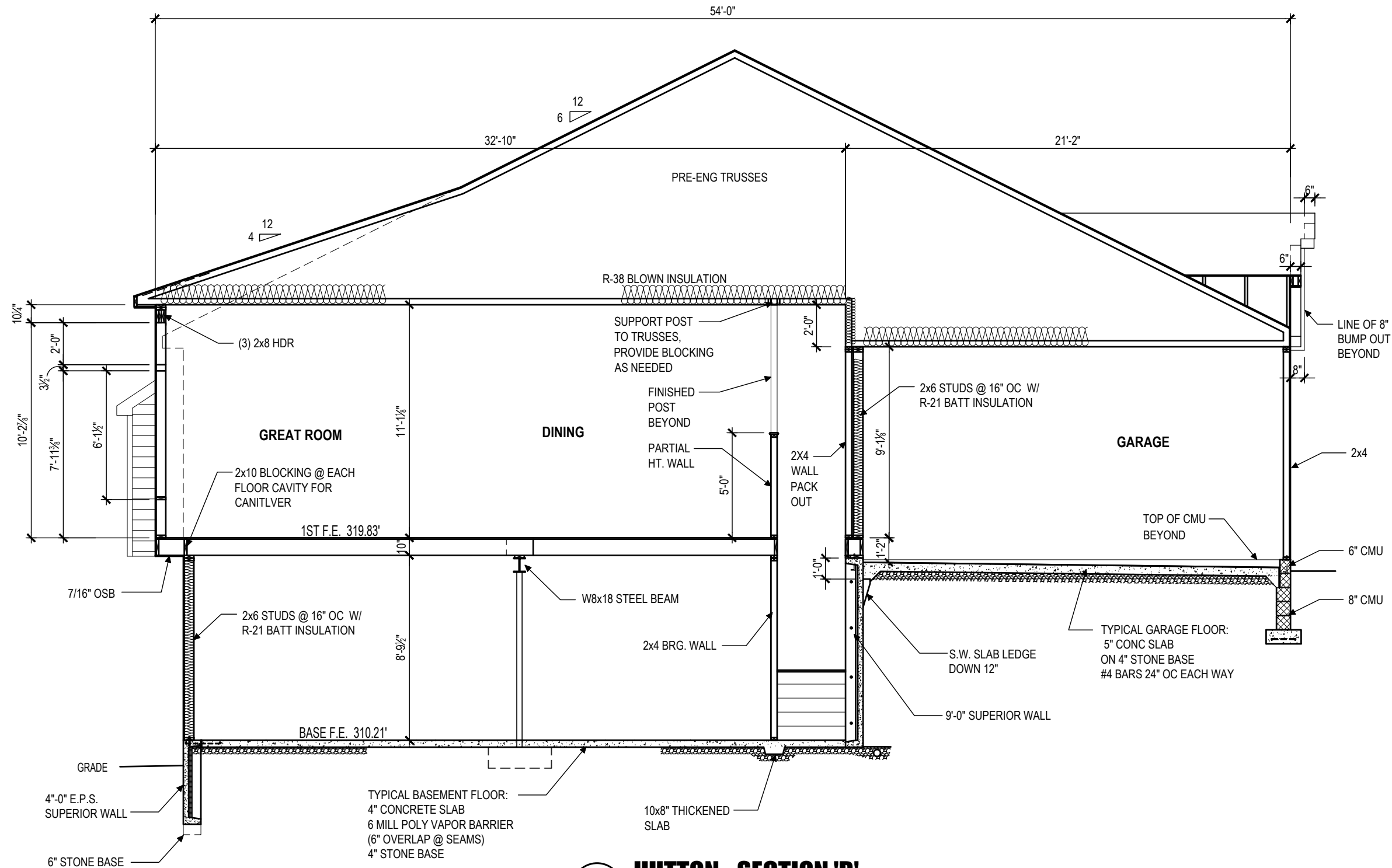
HUTTON - SECTION 'B' SCALE: 3/16"=1'-0"
