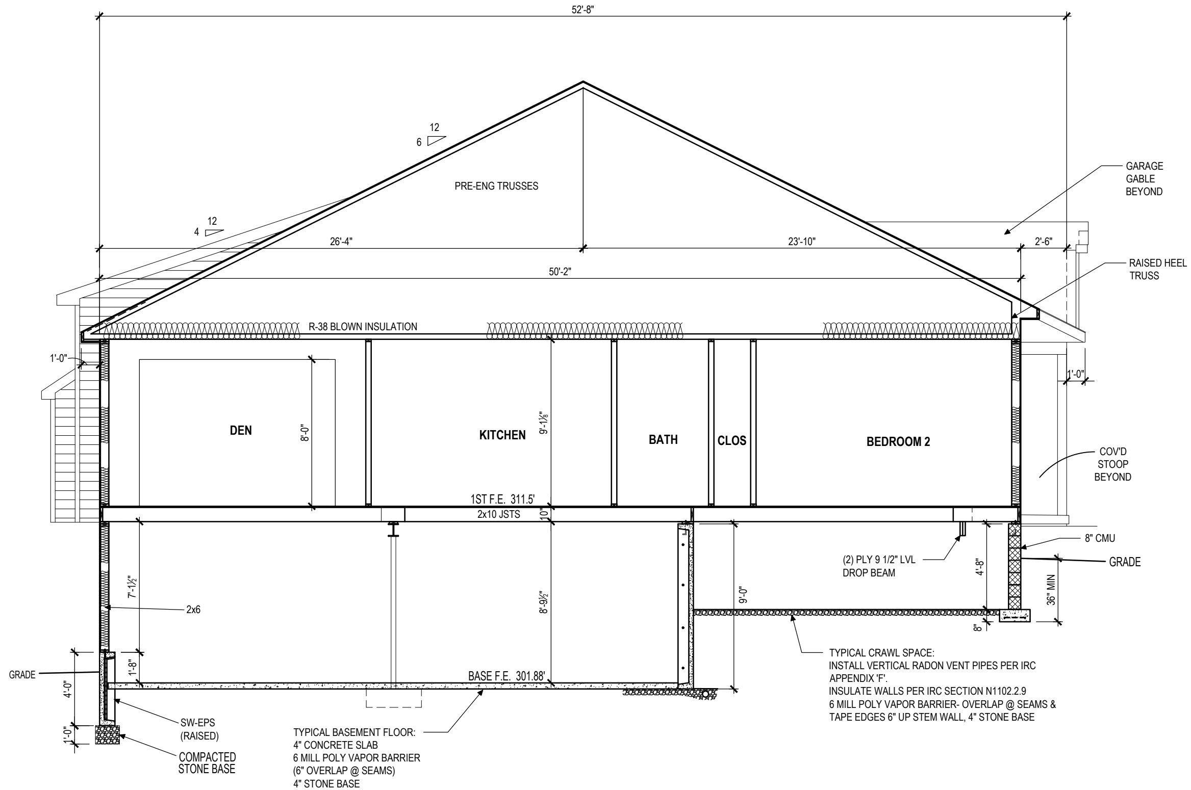
HUTTON - SECTION 'A' SCALE: 3/16"=1'-0"
