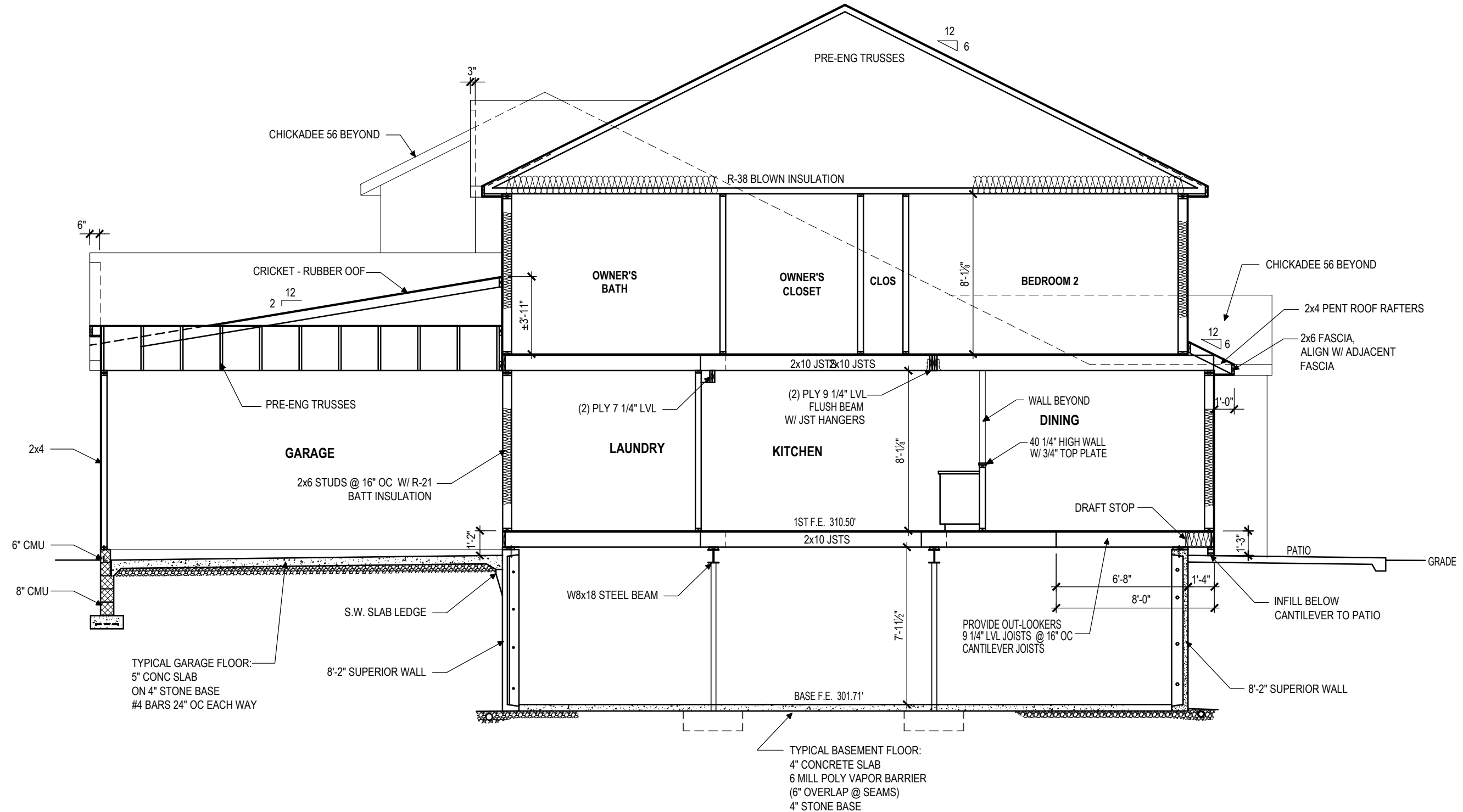
UNIT #57 DAWN - SECTION SCALE: 3/16"=1'-0"
