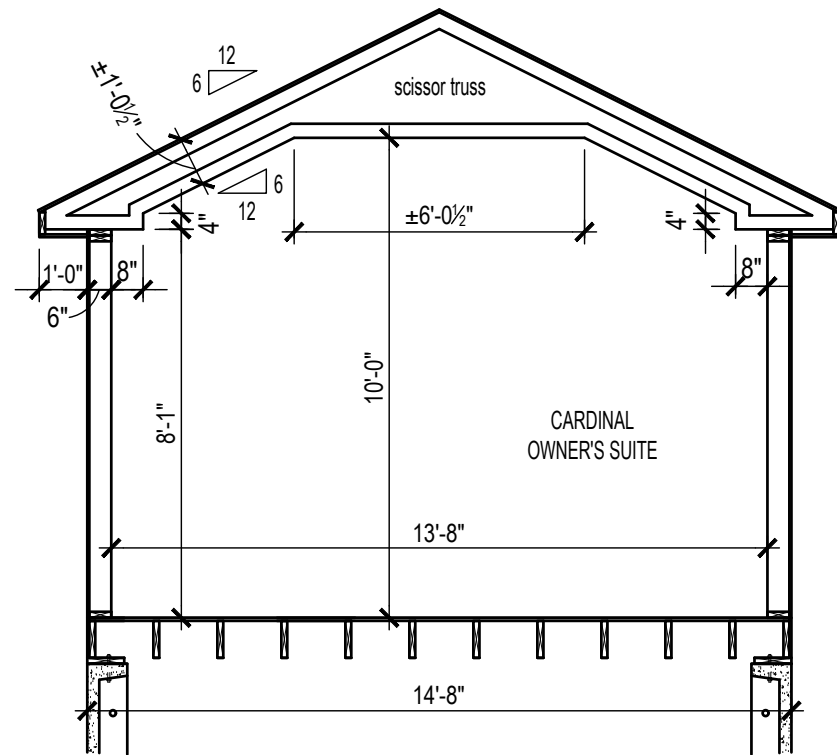
2 A507 OWNER'S SUITE SECTION SCALE: 1/4"=1'-0"
