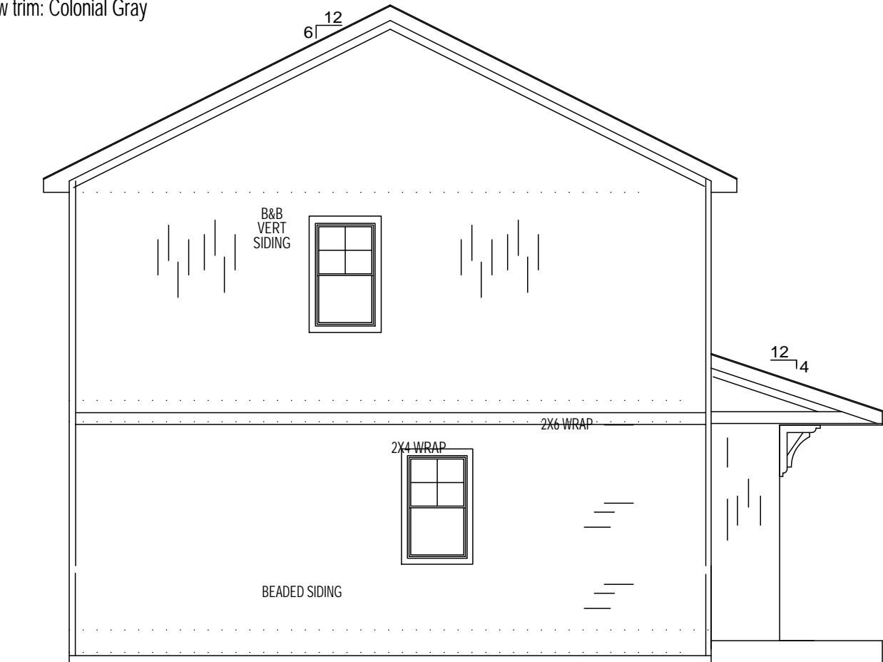
LEFT ELEVATION
