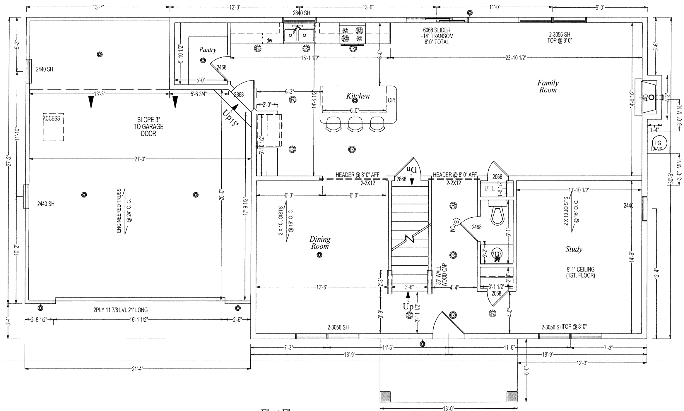
First Floor 9' 1" CEILING TOP OF WINDOWS AT 7' 11 1/2" AFF
