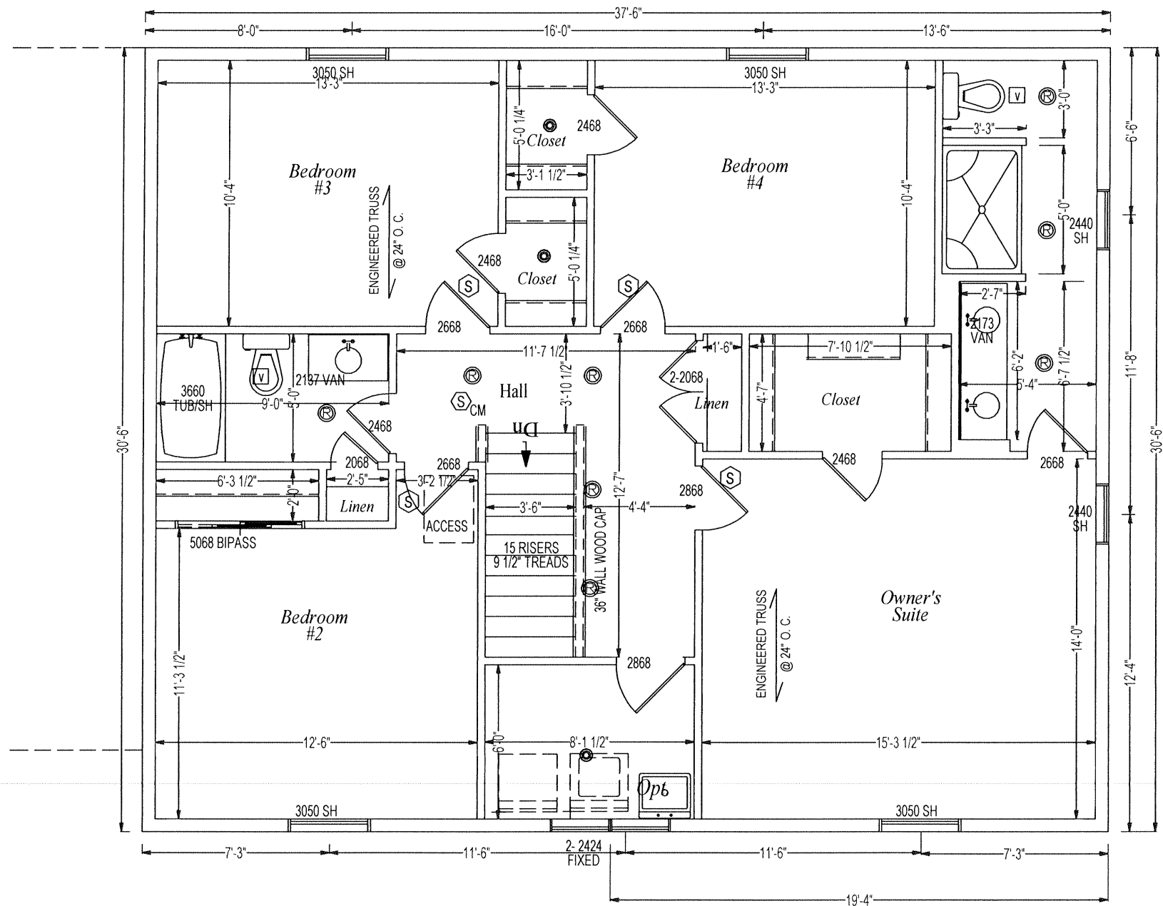
Second Floor
