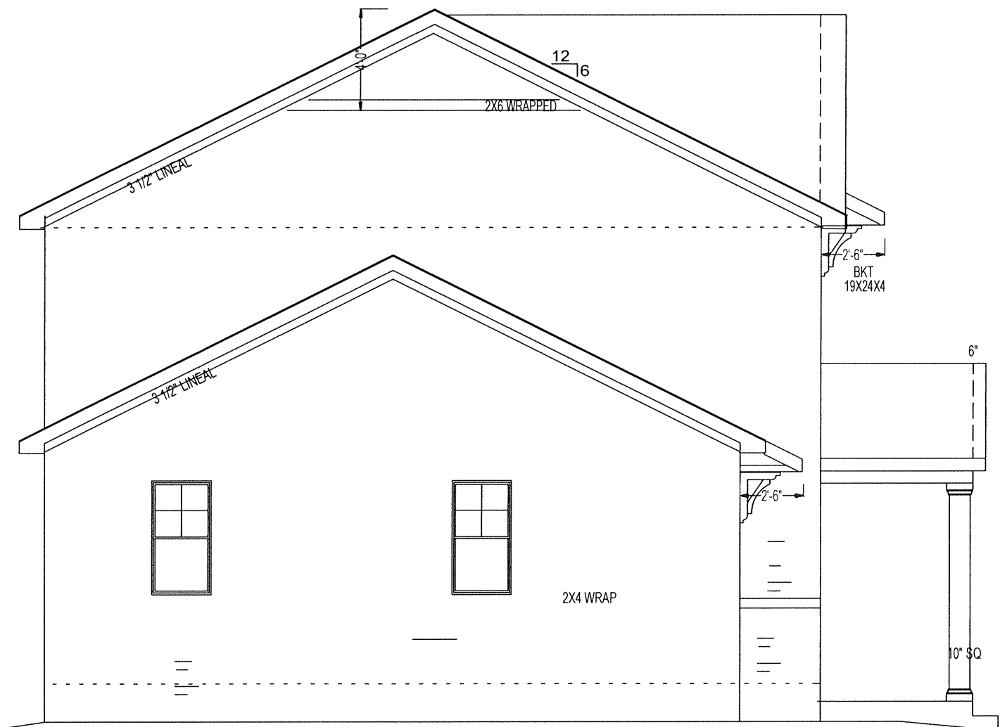
EAST ELEVATION
