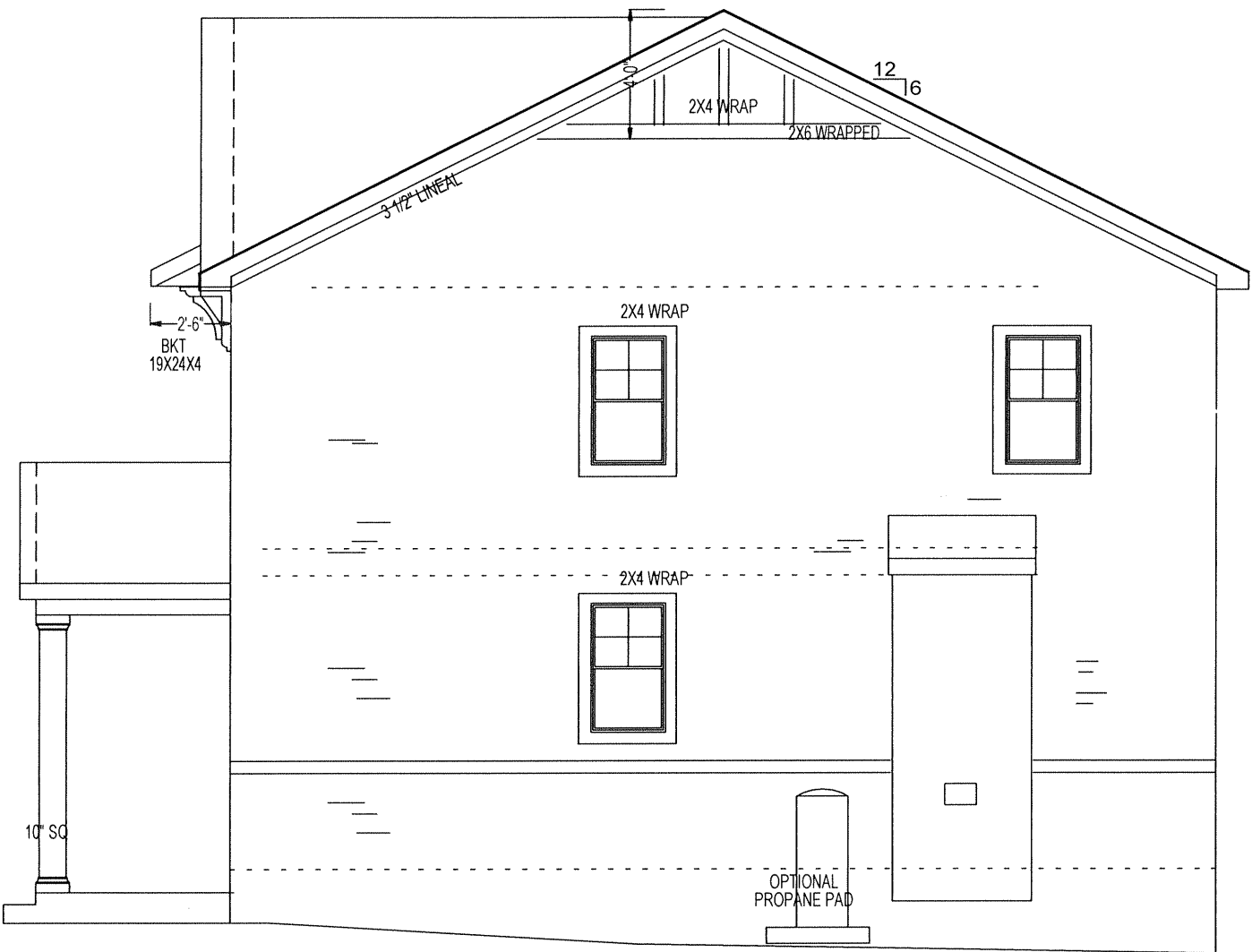
WEST ELEVATION
