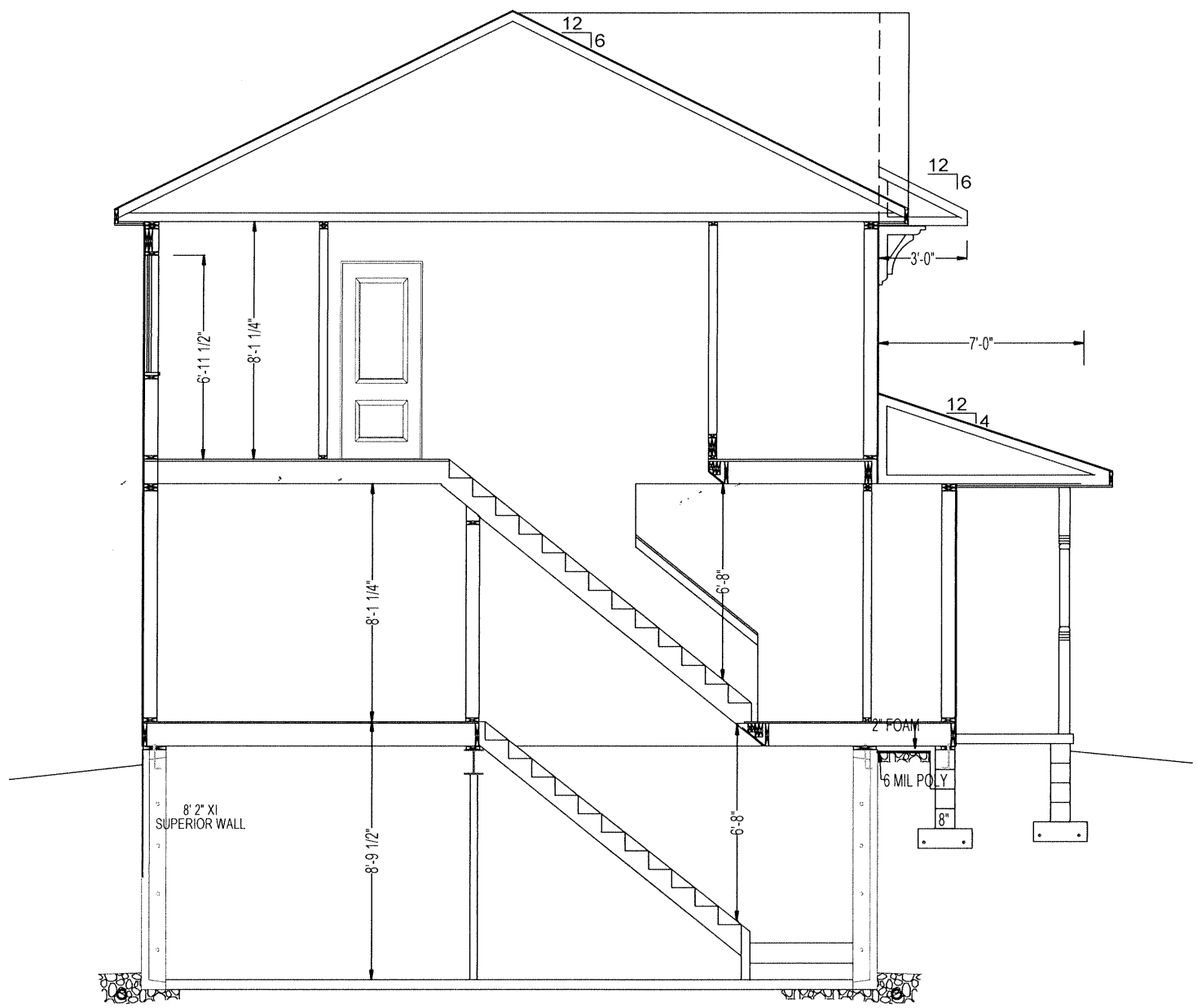
SECTION AA
