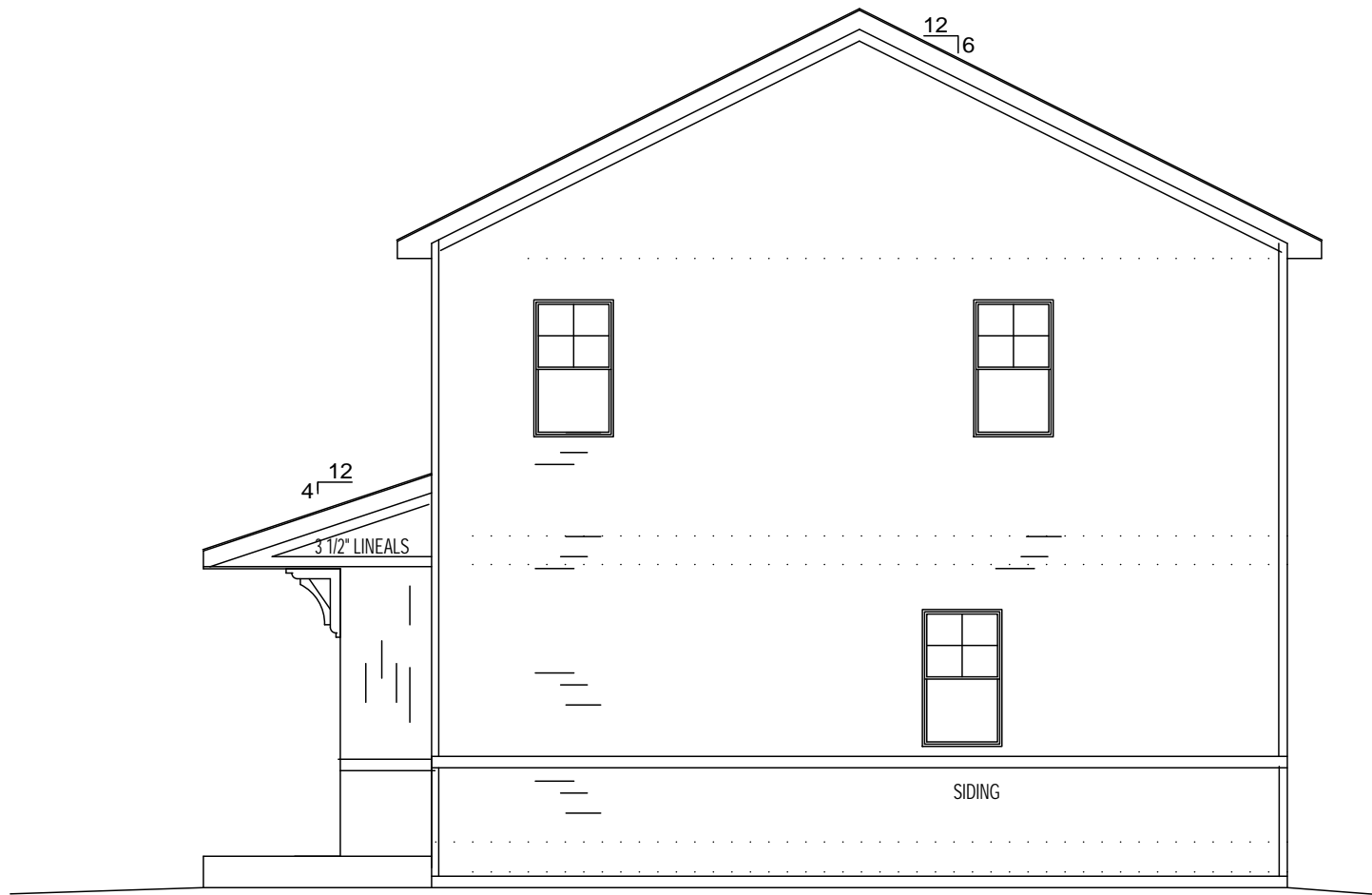
LEFT ELEVATION
