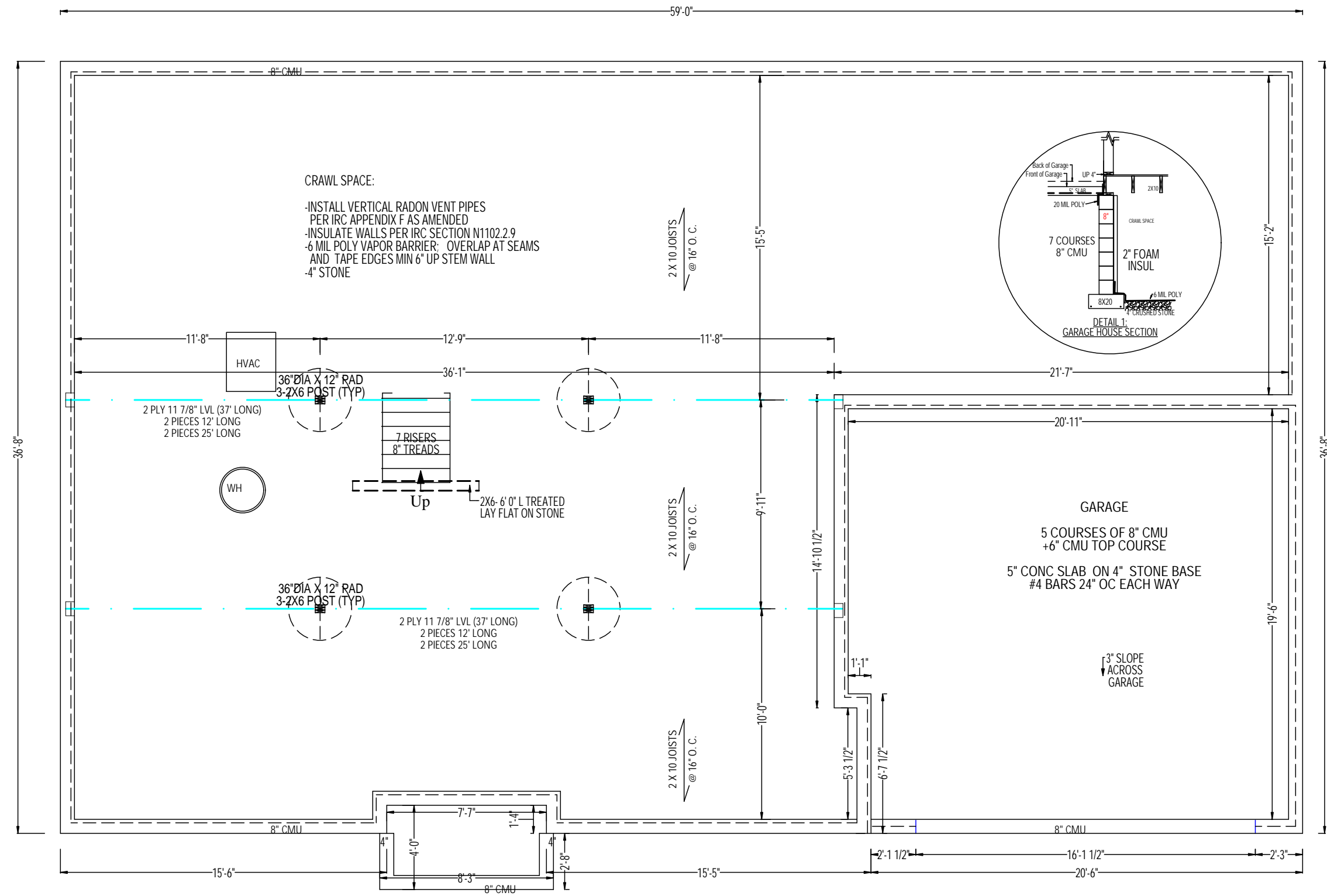
FOUNDATION PLAN
