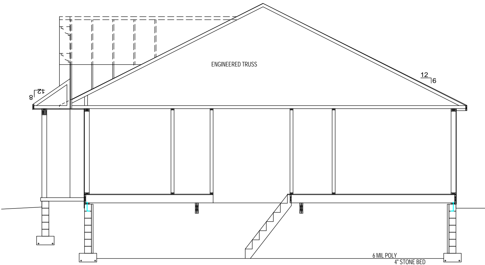
SECTION AA
