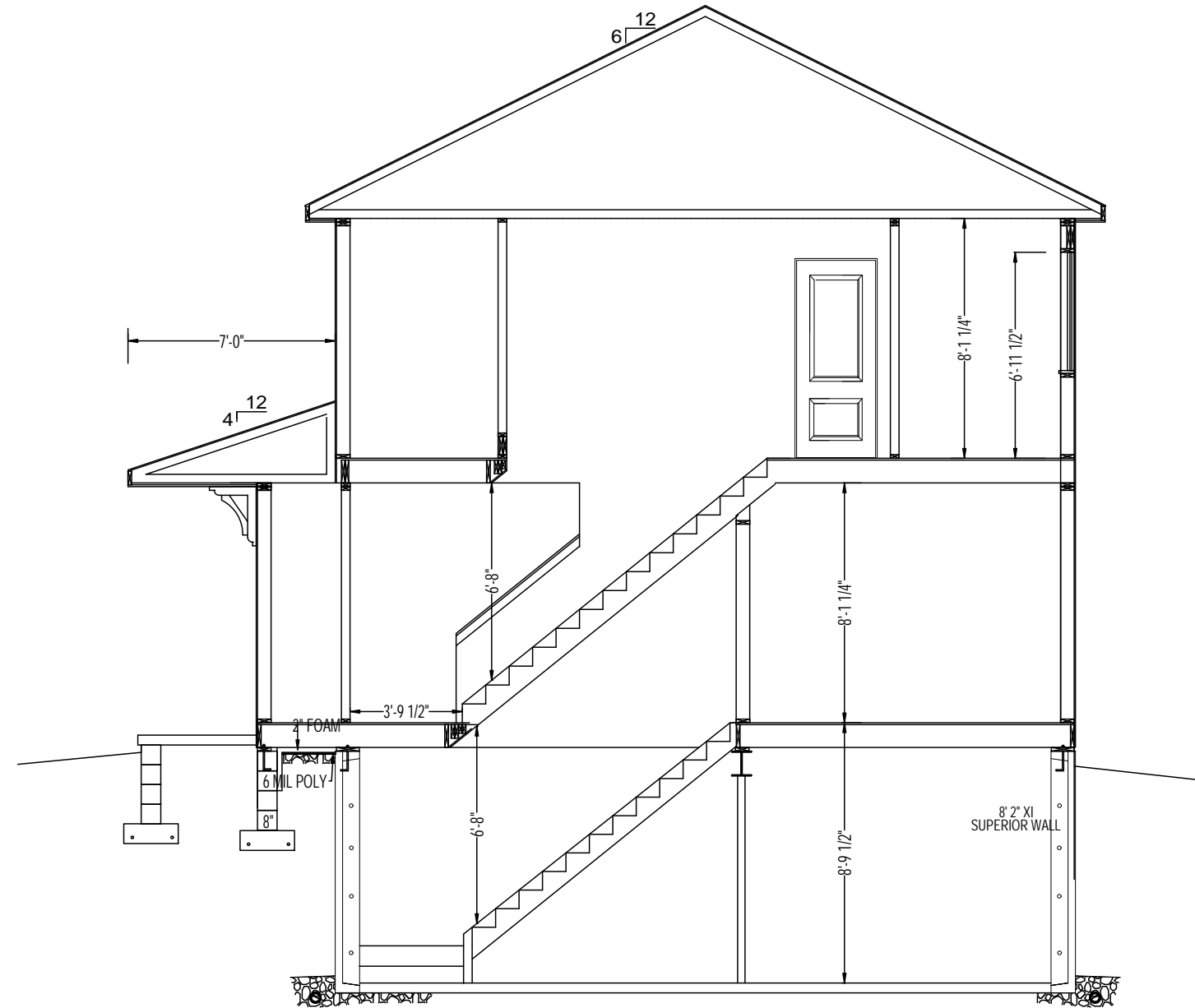
SECTION AA
